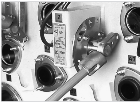
Fault interrupter operating handle
