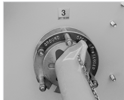
Load break multi-position switch operator
