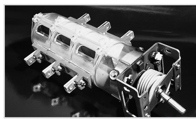
Two position rotary puffer mechanisms
