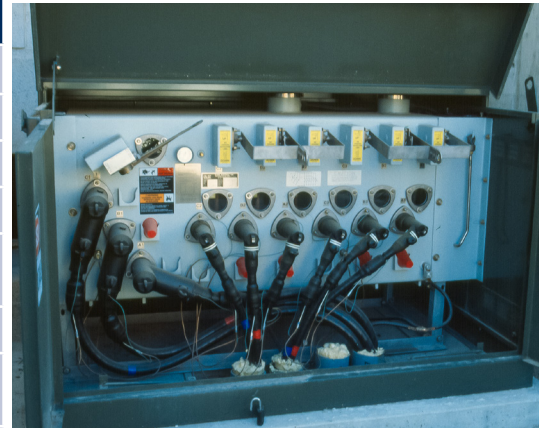
Model PVI-7F with three phase operating handle.
