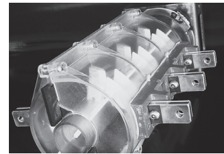
Two position rotary puffer mechanisms.
