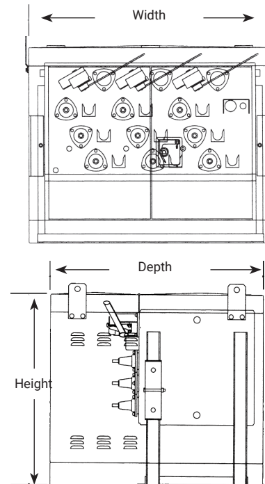
Front access of SPRAM
