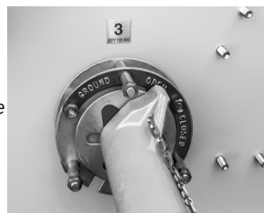
Load break multi-position switch operator.
