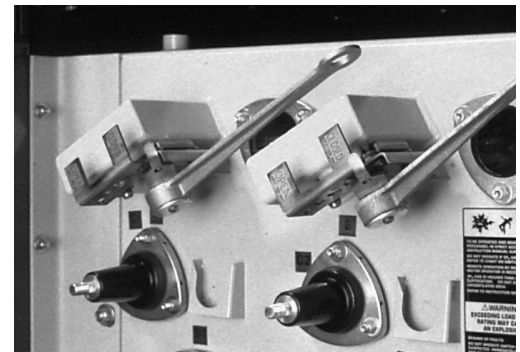
Hookstick operable load break handle
