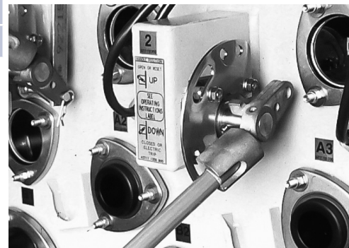
Fault interrupter operating handle.
