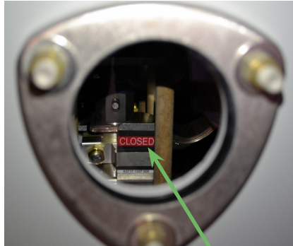
Position indicators provide visible verification of contact position through viewing windows.
