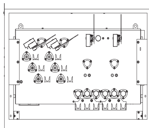
Model PNI-9F Shown with diagonal bushing configuration.
