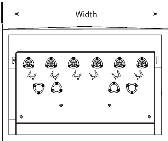
Front view showing source cable entrances.
