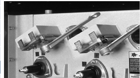
Hookstick operable load break handle.
